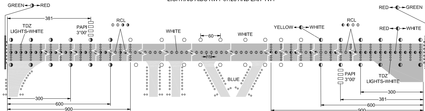
LIGHTING AIDS RWY 07/25 AND EXIT TWY
