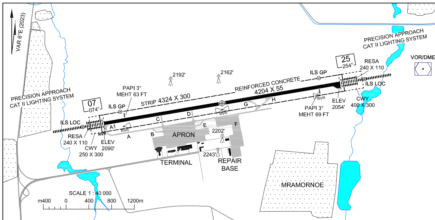
MARKING AIDS RWY 07/25 AND EXIT TWY
