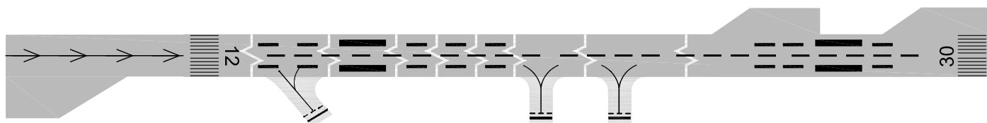
MARKING AIDS RWY 12/30 AND EXIT TWY
